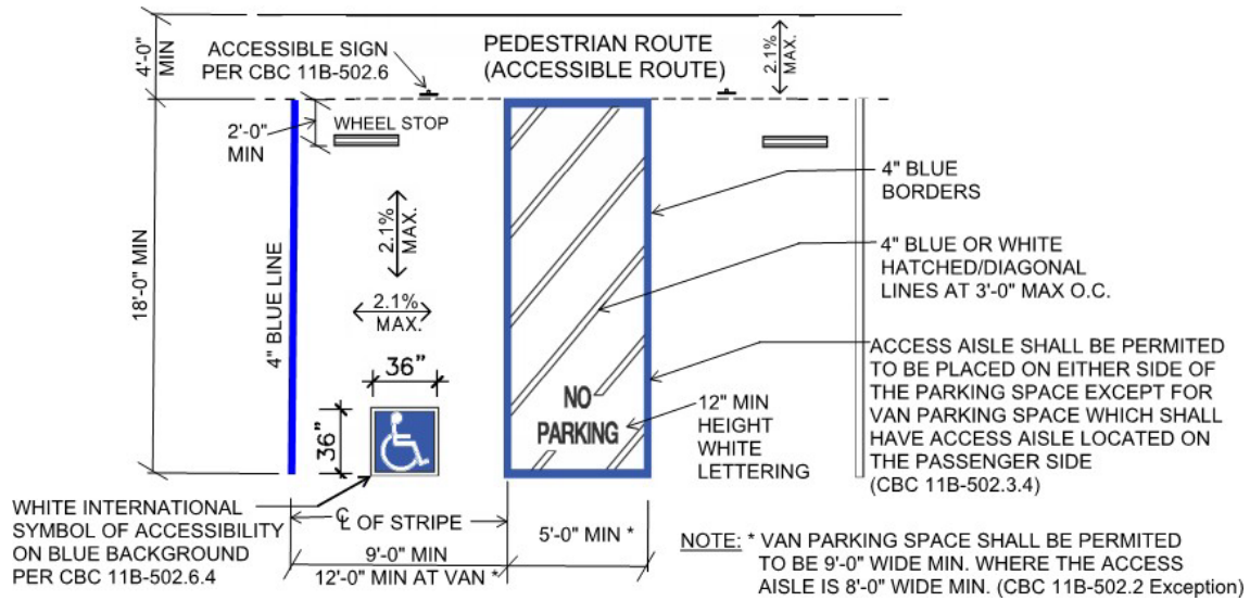
Figure: Single Accessible Parking Stall
