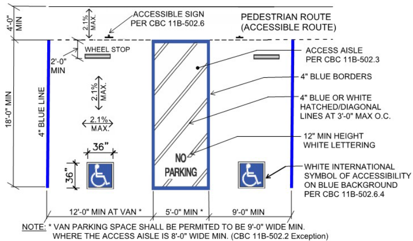
Figure: Double Accessible Parking Stalls
