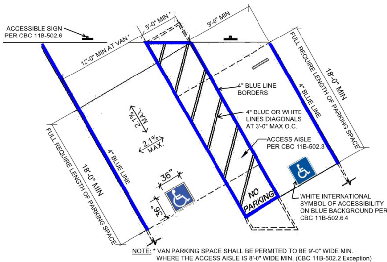
Figure: Diagonal Accessible Parking Stalls
